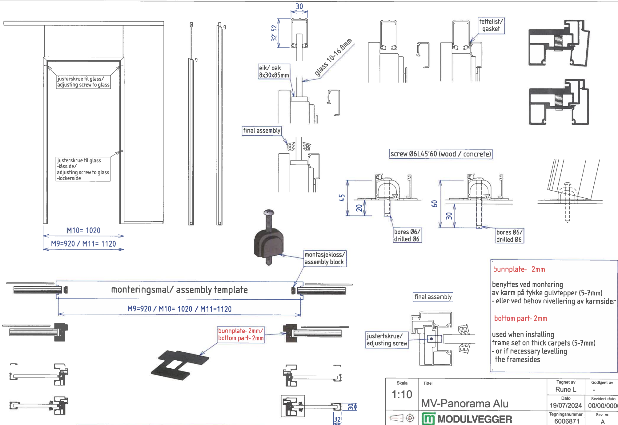
sammenstilling karm/ assembly frame (drawing no. 6006819)
