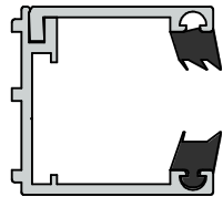
L-PROFIL FOR DEKSEL (10-16,8mm glass)
