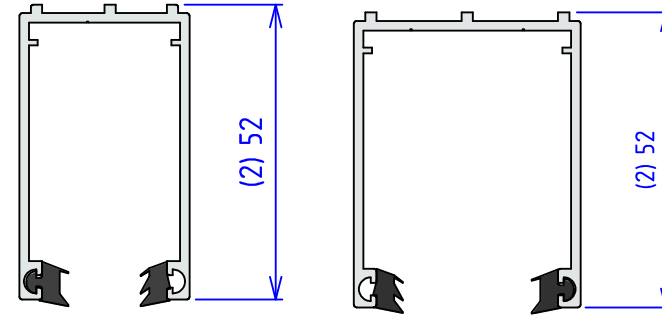
U-PROFIL (20-26mm glass)
