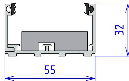
L-PROFIL FOR DEKSEL (35-42mm glass)
